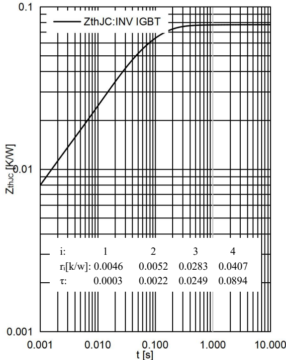
Fig 6. IGBT Transient thermal impedance
