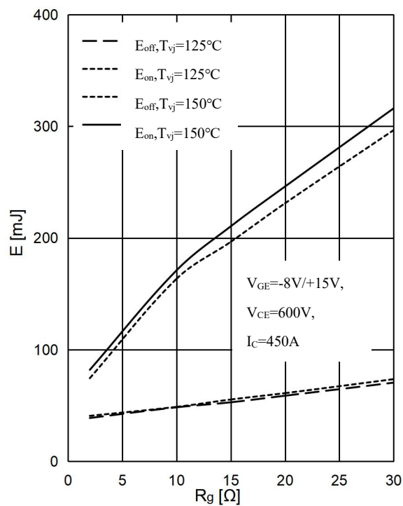
Fig 5. IGBT Switching Loss E_{on} & E_{off} vs. R_g ,
