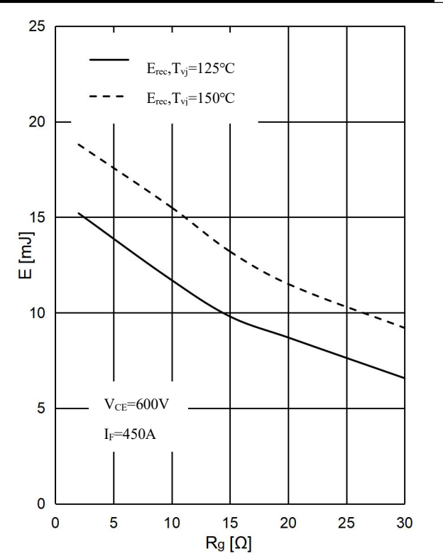
图 10 . 二极管 开关损耗-栅极电阻, Fig 10. Diode Switching Loss E_{rec} vs. R_G
