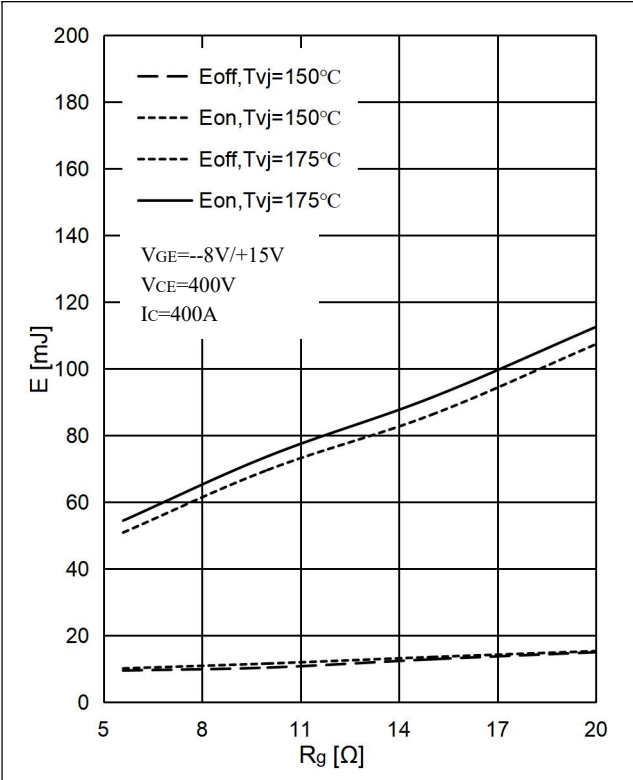
图 5 . IGBT 开关损耗-栅极电阻 Fig 5. IGBT Switching Loss E_{on} & E_{off} vs. R_g
