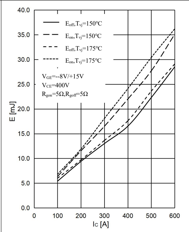
图 4 . IGBT 开关损耗-集电极电流,逆变器 Fig 4. IGBT Switching Loss Eon & Eoff vs. Ic,Inverter
