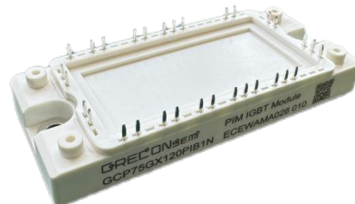
75A/1200V PIM
