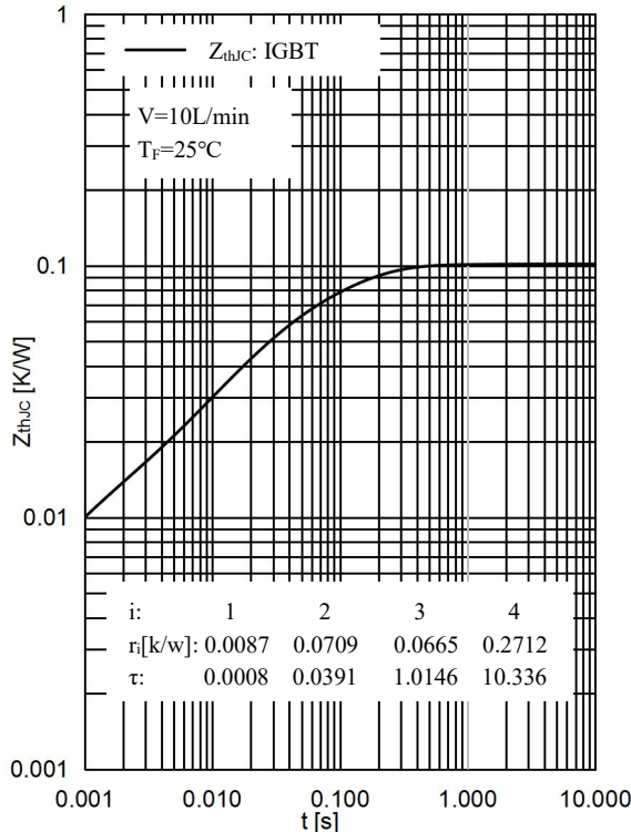
图 6 . IGBT 瞬态热阻抗,T1&T2&T3&T4 Fig 6. IGBT Transient thermal impedance
