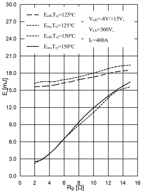
图 5 . IGBT 开关损耗-栅极电阻,T1&T2&T3&T4 Fig 5. IGBT Switching Loss E_{on} & E_{off} vs. R_G
