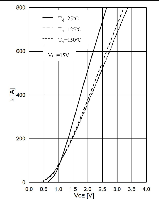
图 1 . IGBT 输出特性,T1&T2&T3&T4 Fig 1. IGBT Output Characteristic,T1&T2&T3&T4
