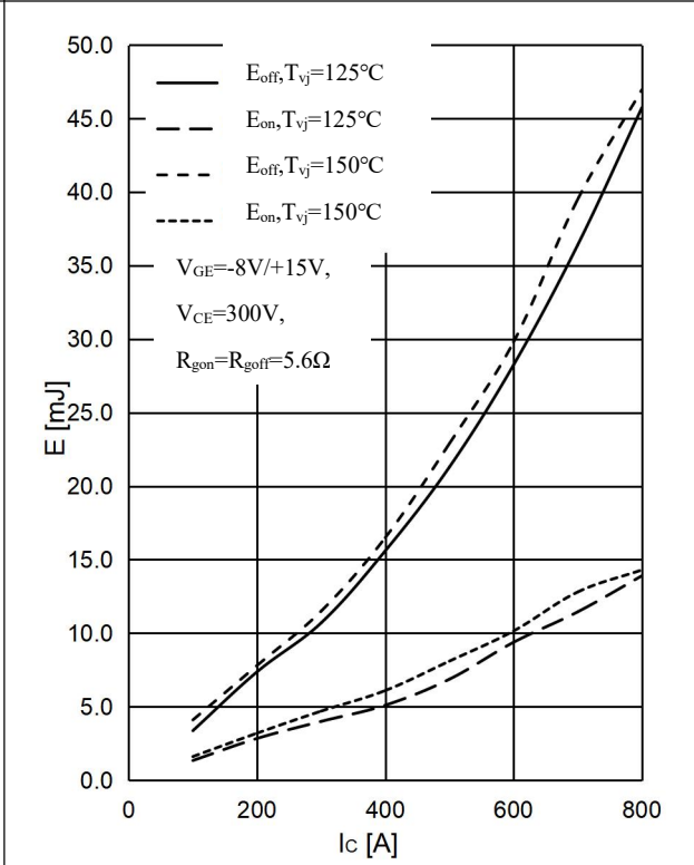
图 4 . IGBT 开关损耗-集电极电流,T1&T2&T3&T4 IGBT Switching Loss Eon & Eoff vs. Ic
