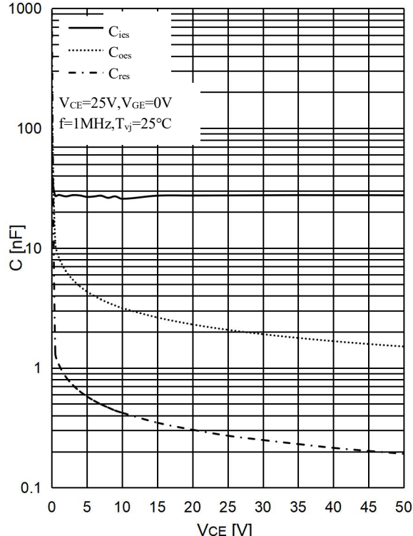
图 8. IGBT 电容特性,T1&T2&T3&T4 Fig 8. IGBT Capacity Characteristic
