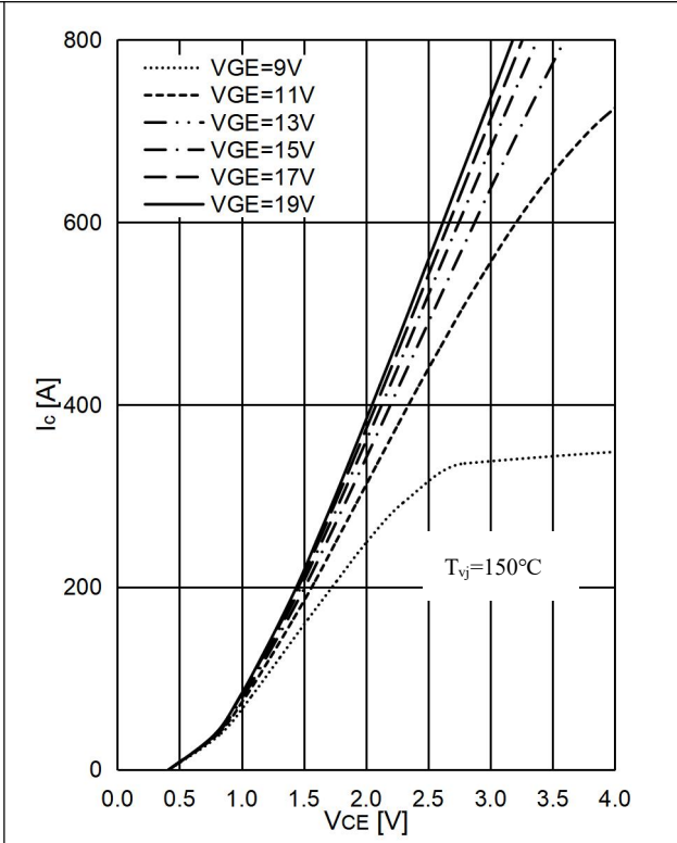
图 2 . IGBT 输出特性,T1&T2&T3&T4 Fig 2. IGBT Output Characteristic,T1&T2&T3&T4
