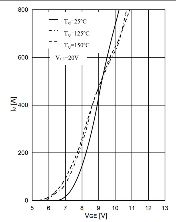
图 3 . IGBT 转移特性,T1&T2&T3&T4 Fig 3. IGBT Transfer Characteristic
