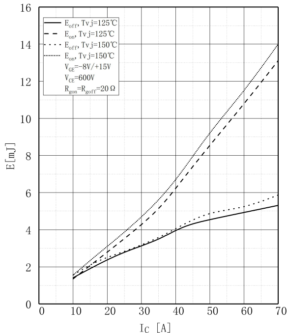
图 4 . IGBT 开关损耗-集电极电流,逆变器 Fig 4. IGBT Switching Loss E_{on} & E_{off} vs. I_C , Inverter
