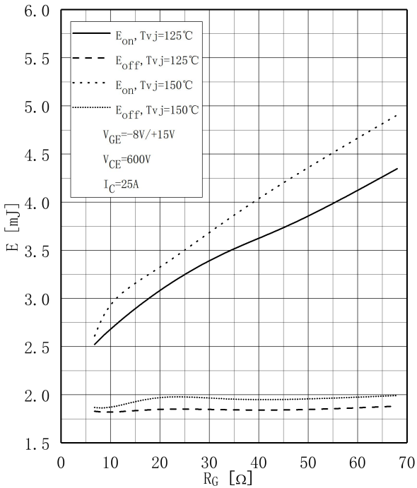
图 5 . IGBT 开关损耗-栅极电阻,逆变器 Fig 5. IGBT Switching Loss E_{on} & E_{off} vs. R_G ,Inverter
