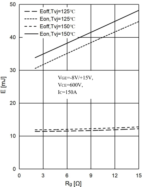
图 5 . IGBT 开关损耗-栅极电阻,逆变器 Fig 5. IGBT Switching Loss E_{on} & E_{off} vs. R_g , Inverter
