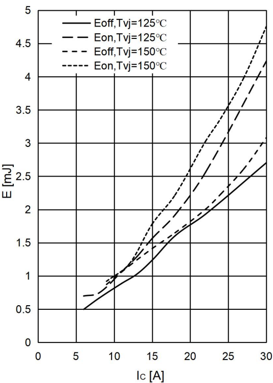
图 4 . IGBT 开关损耗-集电极电流,逆变器 Fig 4. IGBT Switching Loss E_{on} & E_{off} vs. I_c , Inverter
